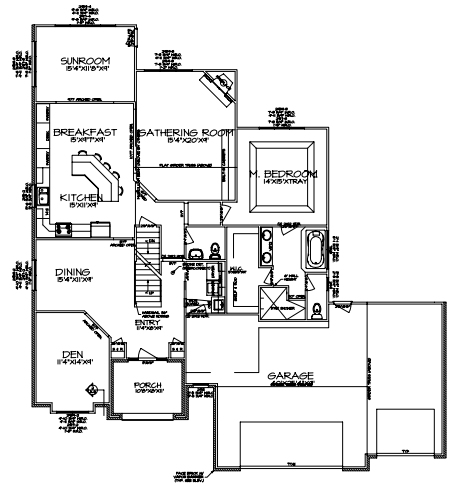
FIRST FLOOR PLAN SCALE: 1/8"=1'-0"
