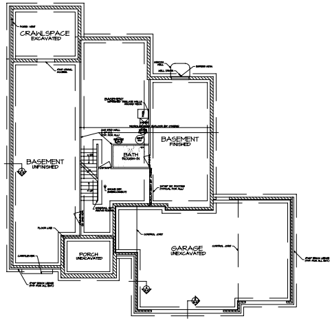
FOUNDATION PLAN SCALE: 1/8"=1'-0"
