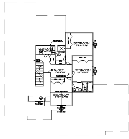
SECOND FLOOR PLAN SCALE: 1/8"=1'-0"
